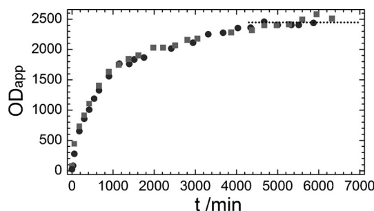
Figure 1. Apparent optical density at 500 nm of 5% aqueous graphene dispersion as a function of sonication time (●, initial preparation; ■, repeat); these values were obtained by diluting sufficiently to obtain absorbances < 2, followed by multiplying these absorbances by their respective dilution factors; adapted from Figure 3 of Ref. [47] with permission.
